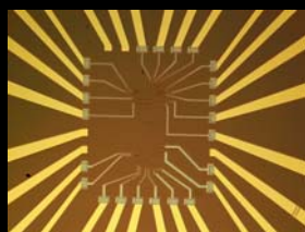
AFM image of the ten SETs on a Si/SiO 2 substrate
